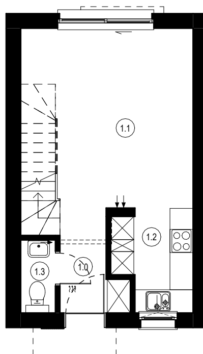
PARTER
